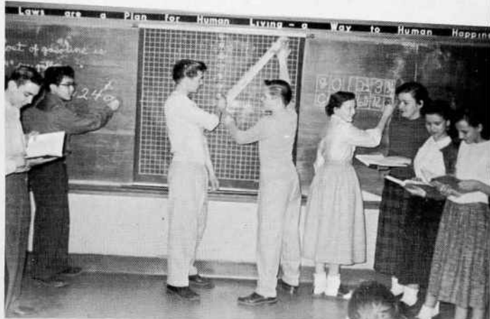
Proving an algebra problem graphically.
